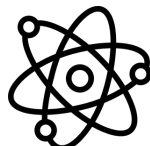
atomic symbol
